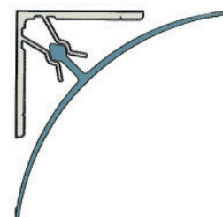
PVC coving section with T aluminium support
